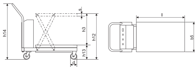
Model: DP30/DP50
